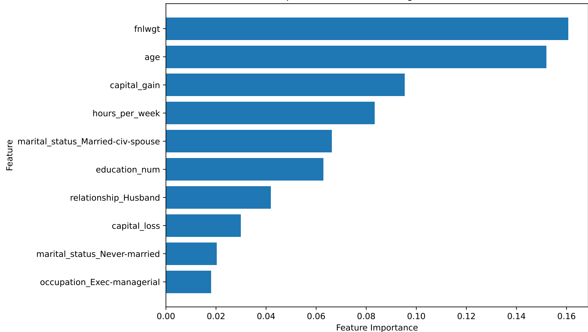
RQ2: Top 10 Features Influencing Income Prediction
